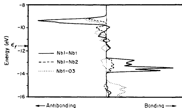
Figure 11. Crystal orbital overlap population (COOP) curve for the Nb1–Nb1 short bond (—), Nb1–O3 (···), and Nb1–Nb2 (---) bonds in the Nb 3 O 6 structure, showing the bonding or antibonding character of the bands across the energy window.
