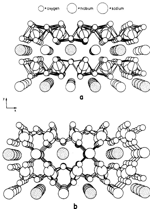
Figure 1. The structure of \text{NaNb}_3\text{O}_5\text{F} seen along z . (a) The coordination polyhedra around \text{Nb2} and the layered structure of the solid are emphasized. (b) The 3D nature of the solid is shown by the Nb–O bonds.
